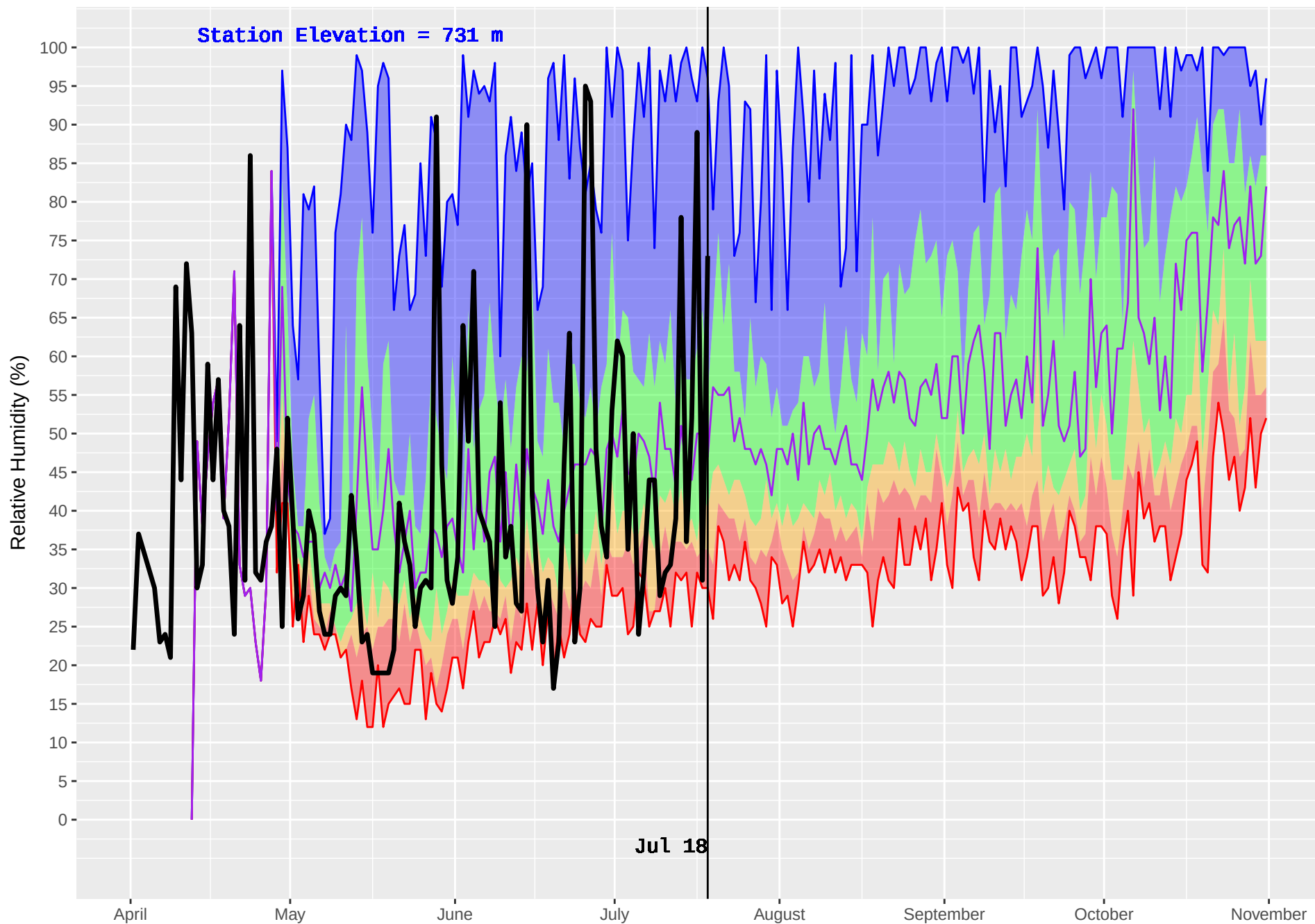
FIRESIDE (440) : Historical (1996–2016) and Current (2018) Daily Relative Humidity
